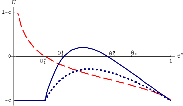
Figure 2: Equilibria with multiple attacks.
