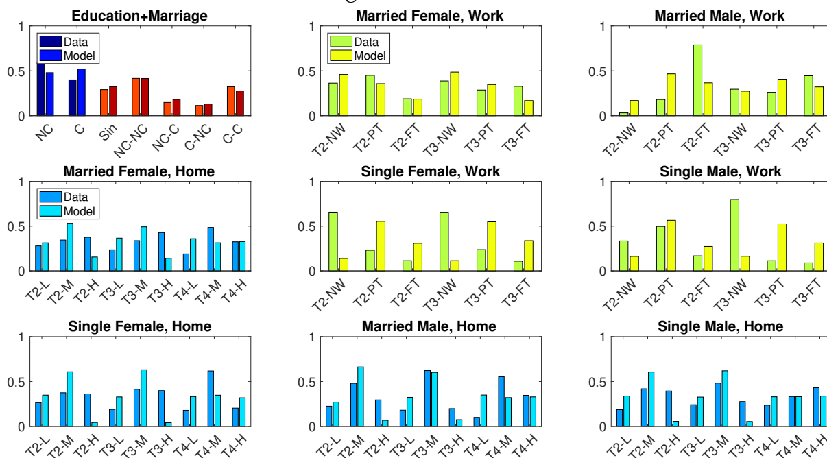
Figure 4: Model Fit
