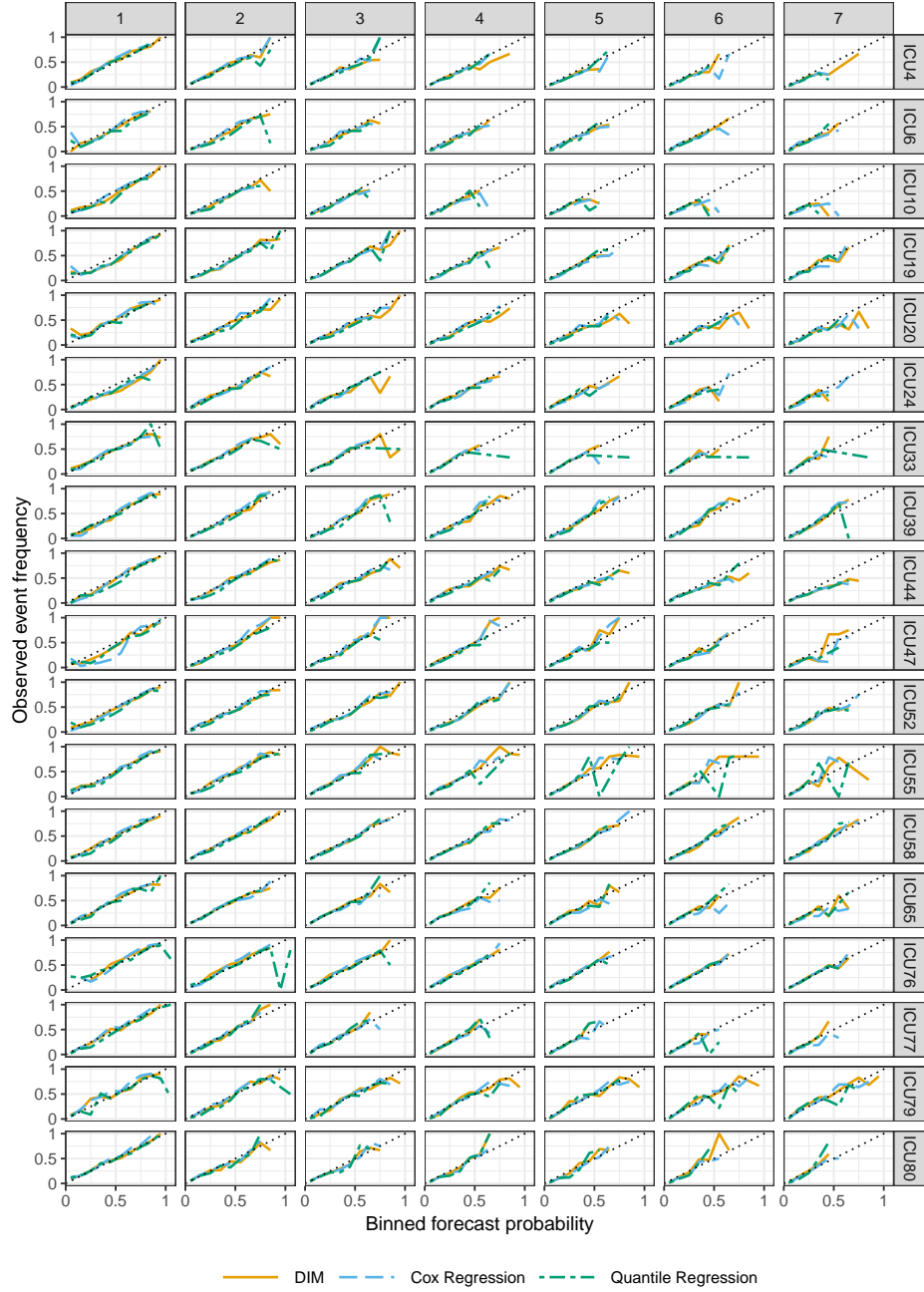
Figure S2: Reliability diagrams of probabilistic forecasts for the predicted probability that the LoS exceeds 1, 2, \dots , 7 days. The forecast probability is grouped into the bins [0, 0.1] , (0.1, 0.2] , \dots , (0.9, 1] . Only bins with more than two observations are included.
