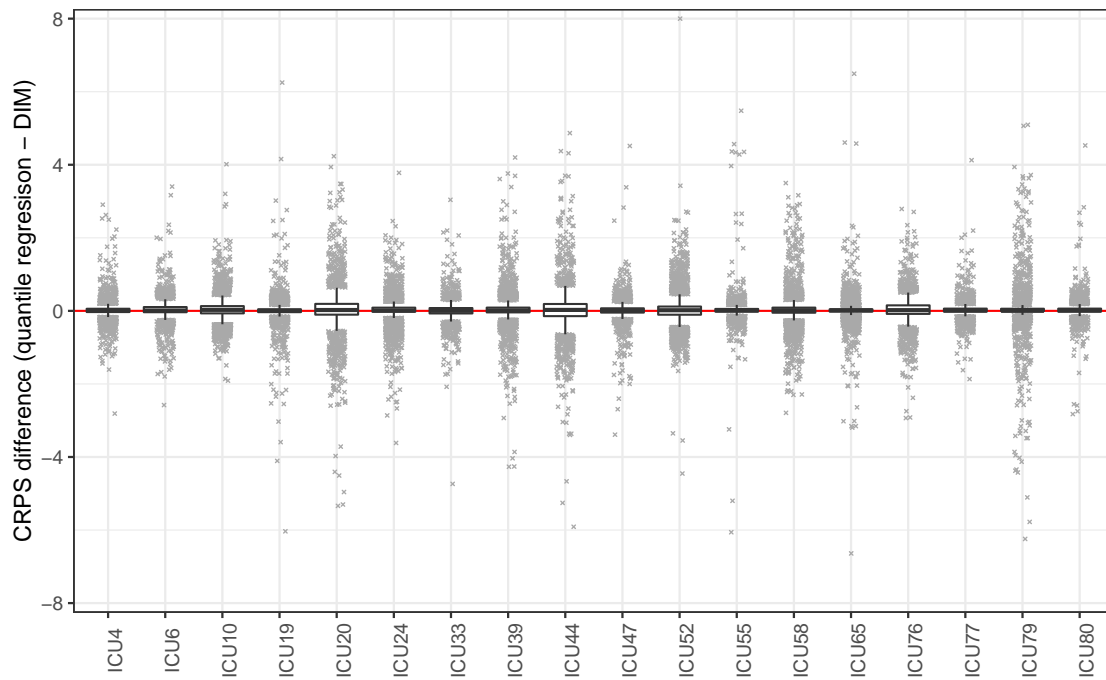
Figure S6: Boxplot of the difference in the CRPS of the quantile regression forecasts and of the DIM forecasts. Outliers are displayed as crosses (with horizontal jitter).
