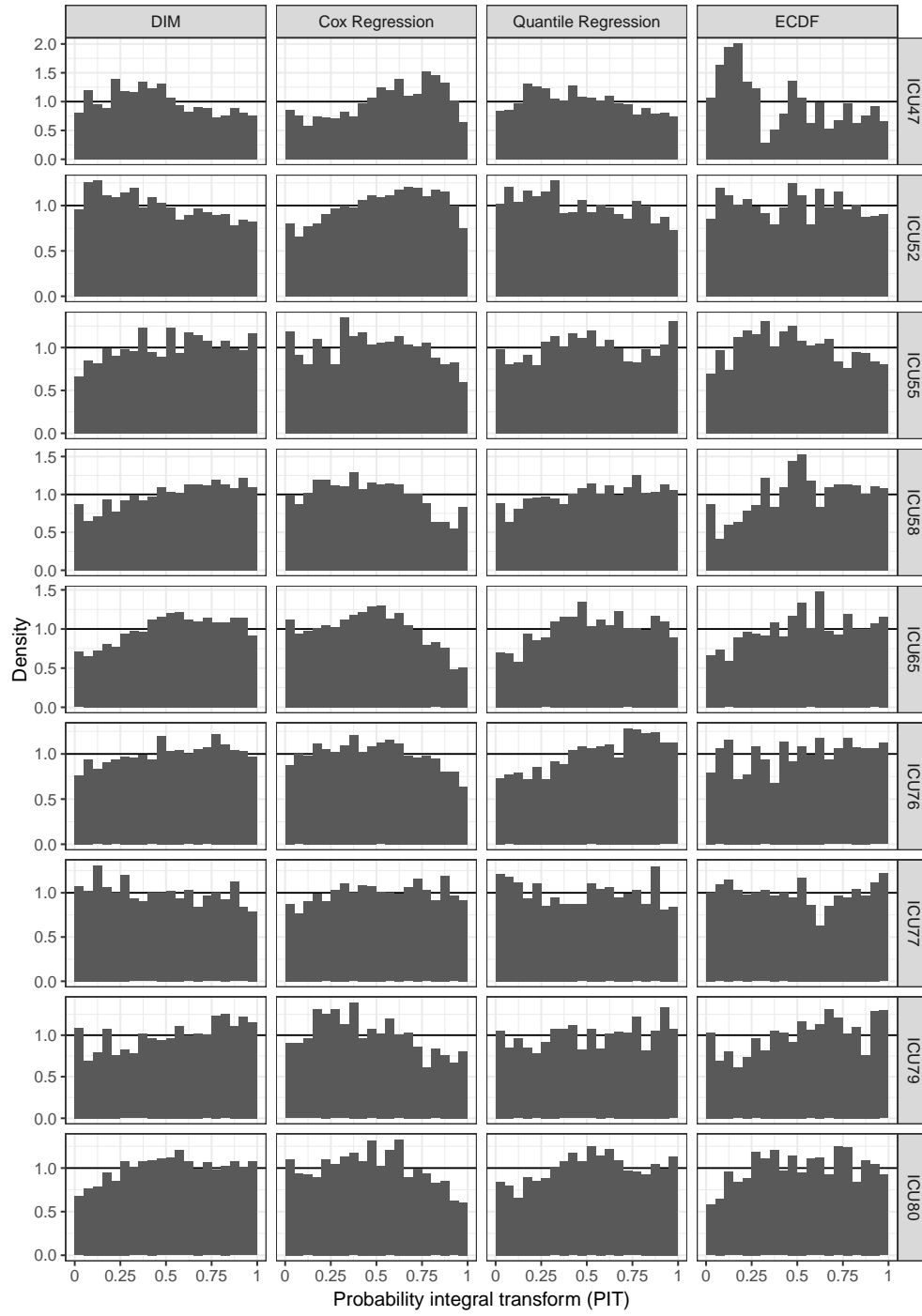
Figure S5: PIT histograms of the probabilistic forecasts with bins of width 1/20 (second half of the ICUs).
