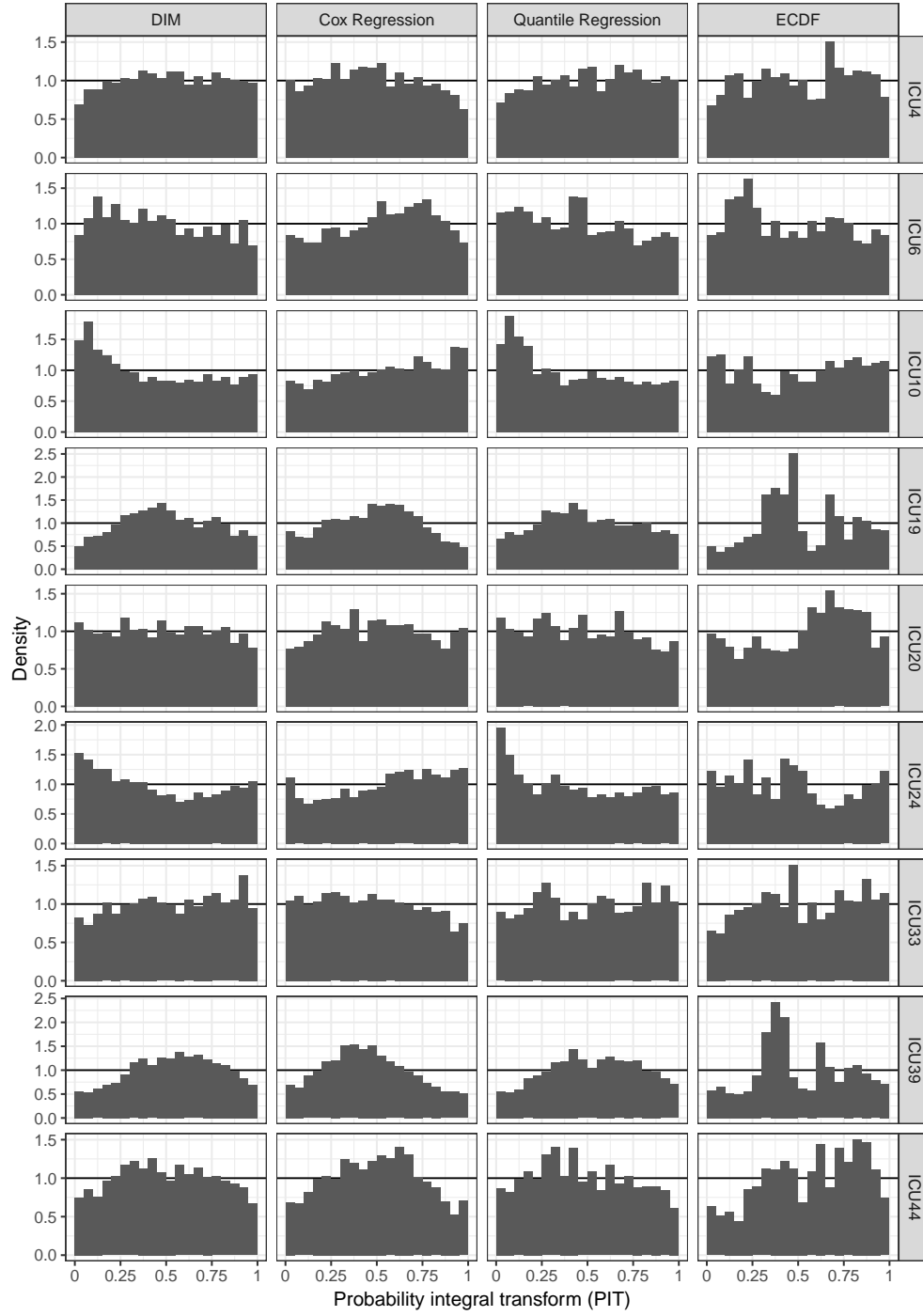
Figure S4: PIT histograms of the probabilistic forecasts with bins of width 1/20 (first nine ICUs).
