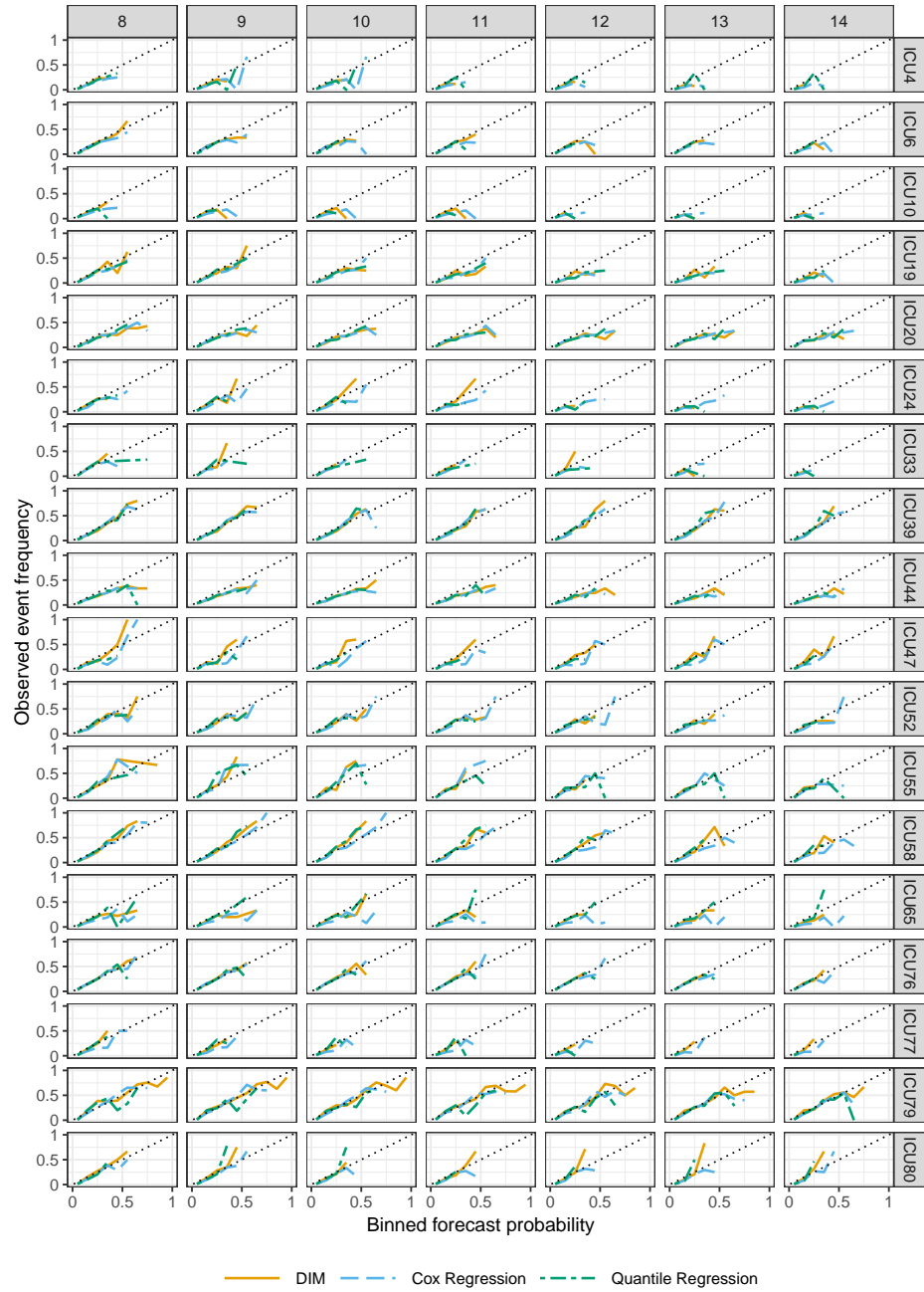
Figure S3: Reliability diagrams of probabilistic forecasts for the predicted probability that the LoS exceeds 8, 9, ..., 14 days. The curves are as specified in Figure S2.
