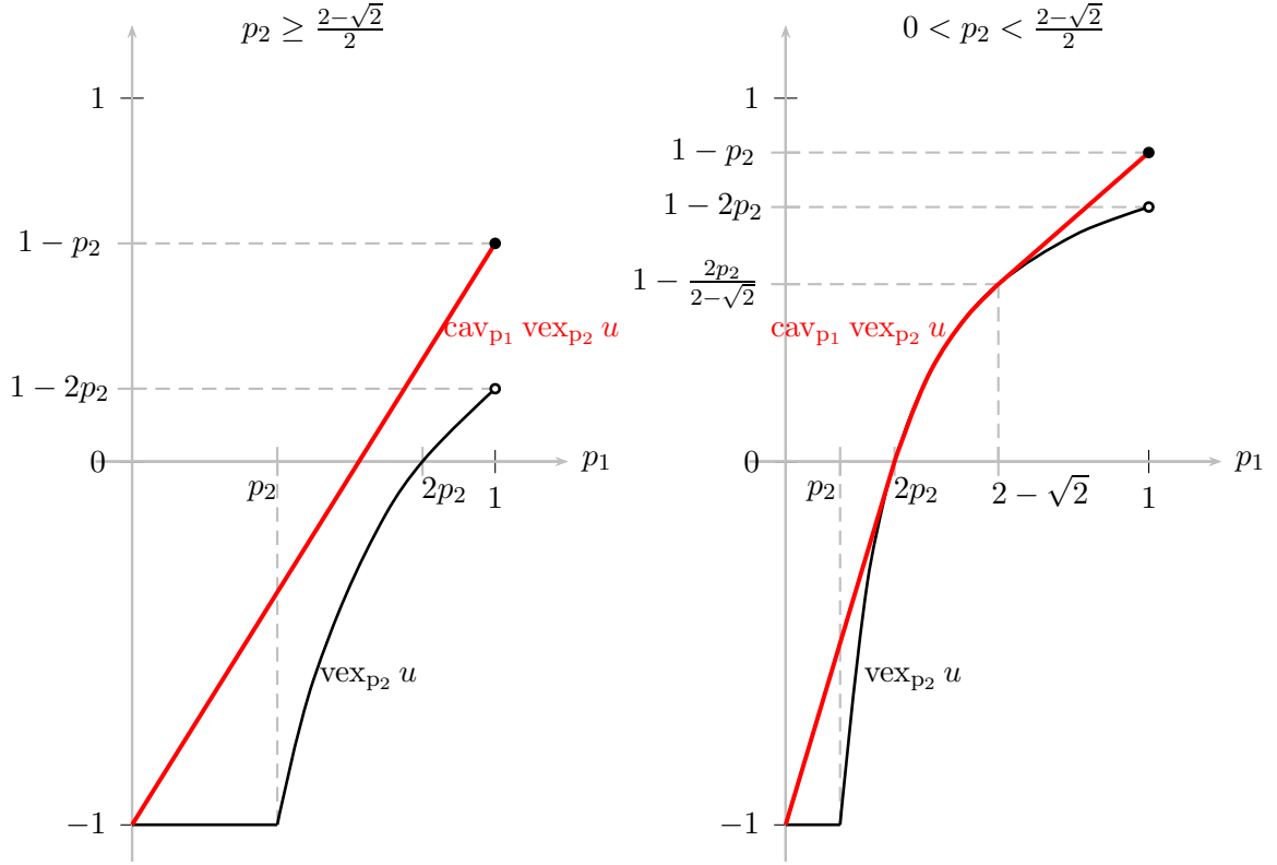
Figure 3: Concavification of \text{vex}_{p_2} u(p_1, p_2) if p_2 \geq \frac{2-\sqrt{2}}{2} (left figure) and 0 < p_2 < \frac{2-\sqrt{2}}{2} (right figure).
