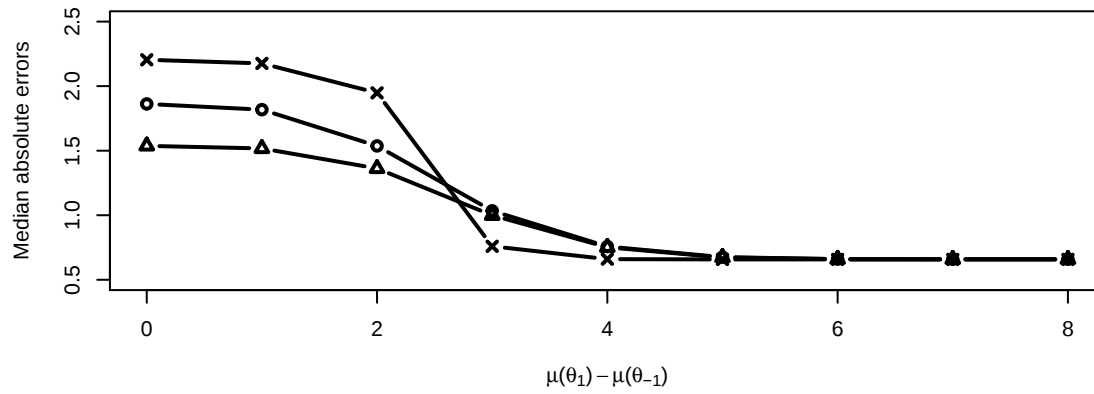
Figure 4: Median absolute error of estimators of \mu(\hat{\theta}) in cases with 2, 10, and 50 policies.
