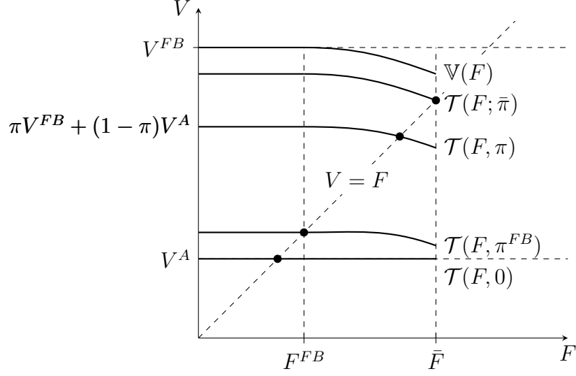
Figure 1: Determination of the fixed point of \mathcal{T}(F; \pi) = \pi \mathbb{V}(F) + (1 - \pi)V^A for different values of \pi . Drawn for \beta > \beta^{FB} , where \beta^{FB} is defined in Proposition 1 and assuming \mathbb{V}(\bar{F}) > \bar{F} (Lemma A.2 verifies that F > F^{FB} if \beta^{FB} < \beta ); if \beta < \beta^{FB} , then F^{FB} < V^A .
