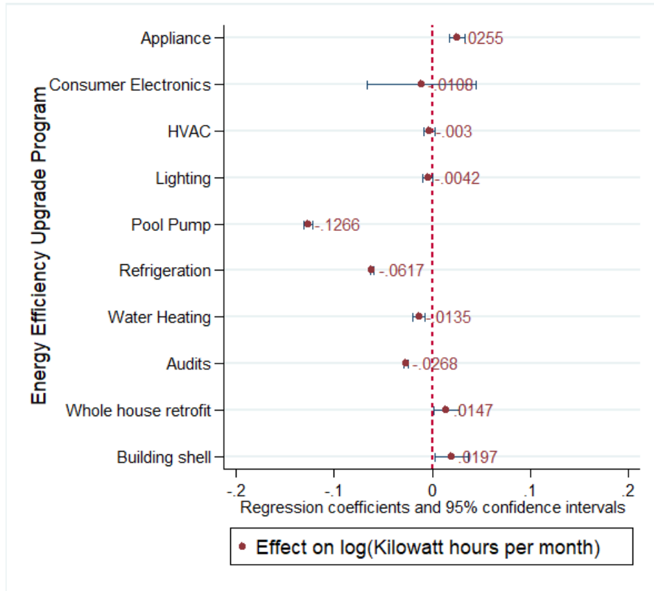
Figure 4: Energy Efficiency Overall Regression Result
