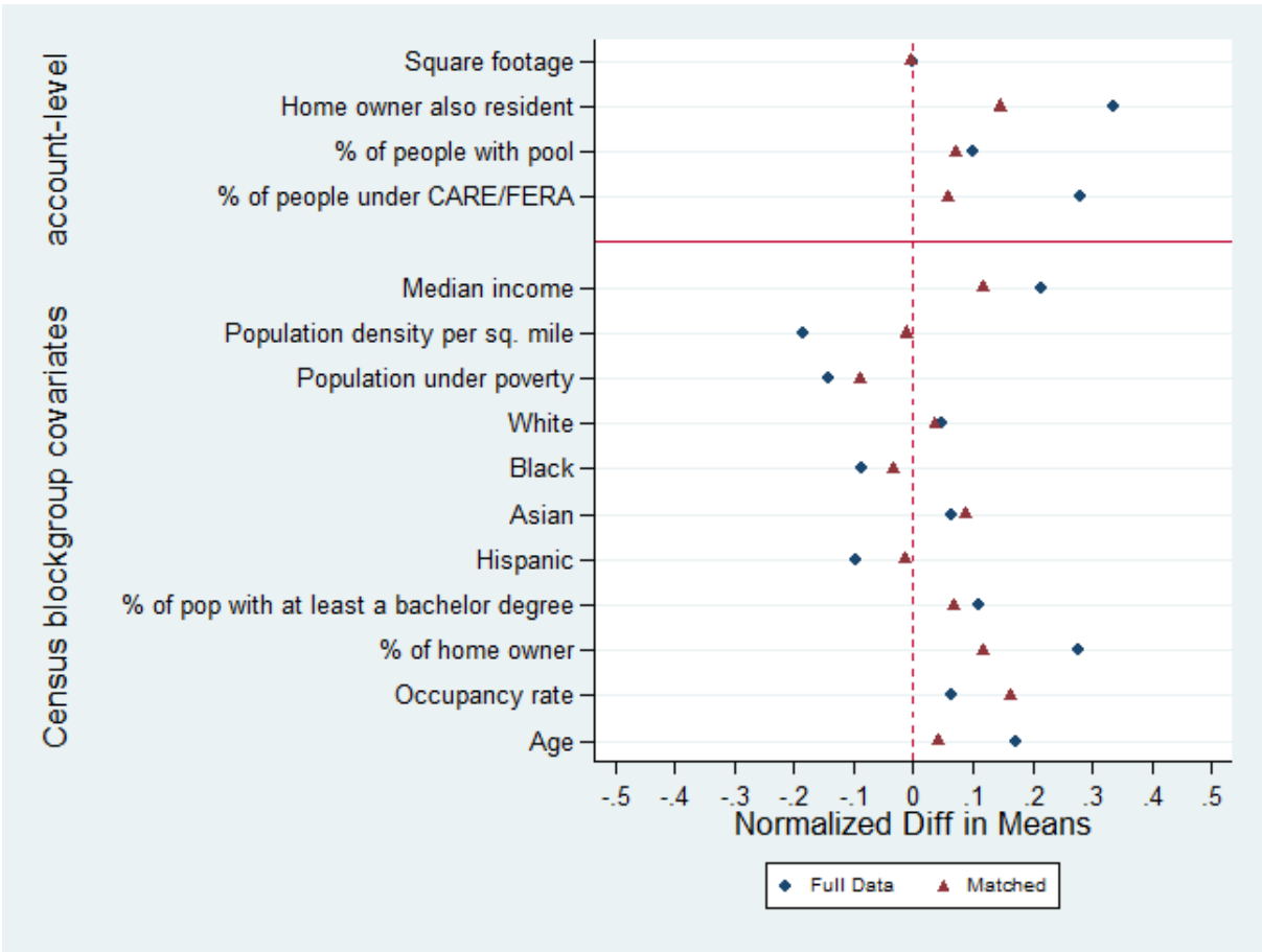
Figure 2: Changes in Normalized Differences after Matching
