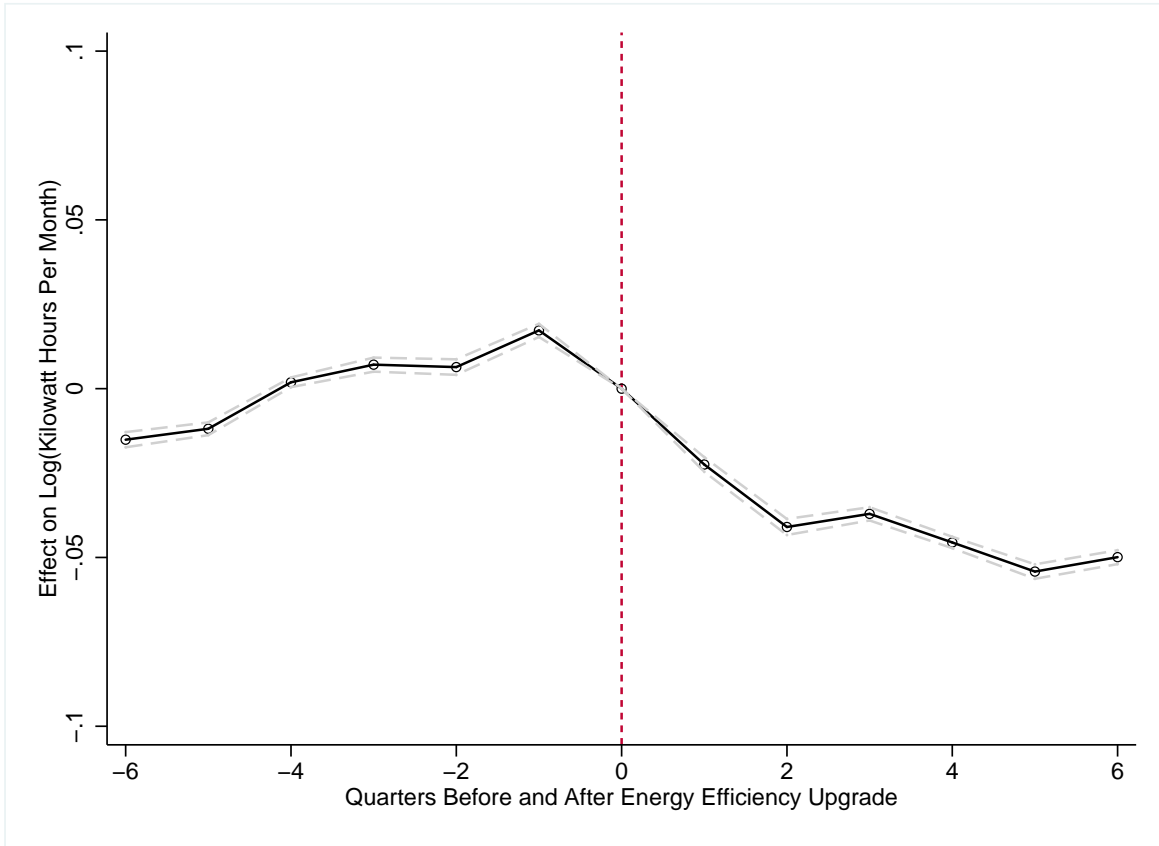
Figure 3: Impact of Energy Efficiency Programs on Electricity Consumption
