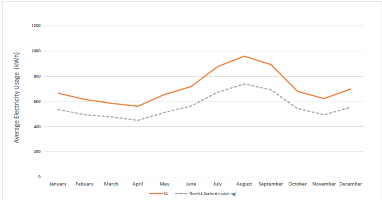
Figure 1: Average Electricity Consumption Pattern among Energy Efficiency Program Participants and Non-participants
