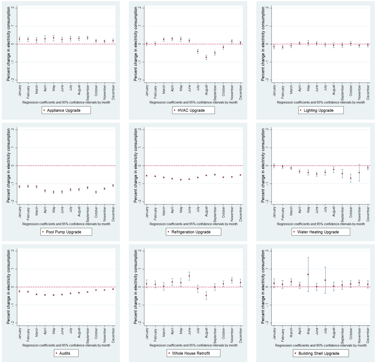
Figure 5: Percent Change in Electricity Consumption by Product and Month
