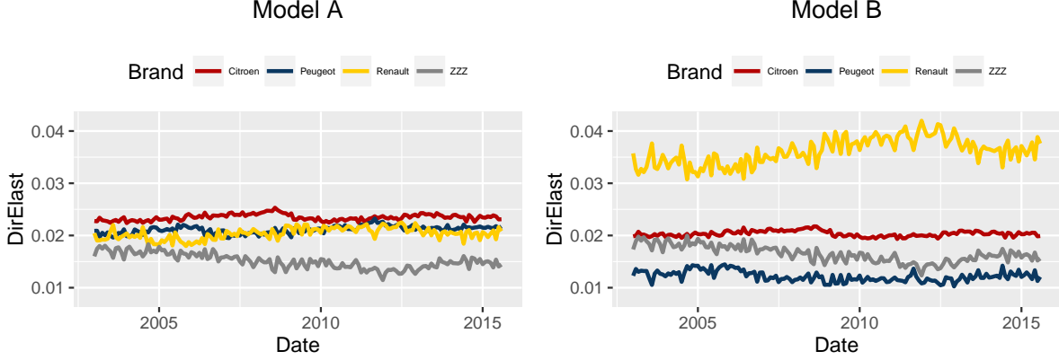
Figure 4: Direct elasticity of S_{jt} relative to M_{j,t-1} across time
