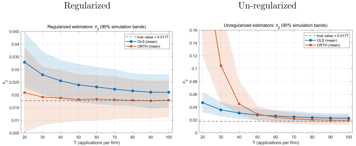
Figure 2: Monte Carlo estimates of \theta_2 as a function of T . Solid lines show the mean across simulations for OLS and ORTH; the dashed line is the true value; shaded regions are 90% simulation bands.
