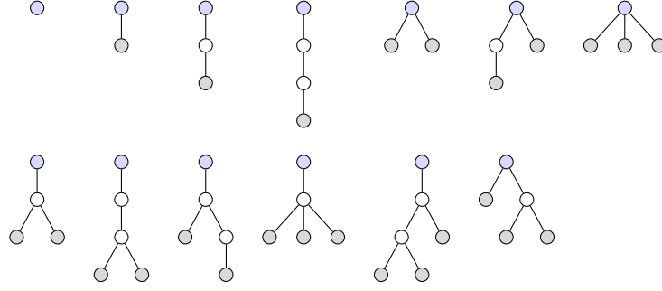
Figure 4: The thirteen elements of \mathcal{T}_3 . The first row shows the seven trees in which every non-root node has at most one child — these correspond to the terms of the affine moment function \psi_{\text{aff}}^{(3)} . The second row shows the six correction trees, each containing at least one non-root node with two or more children.
