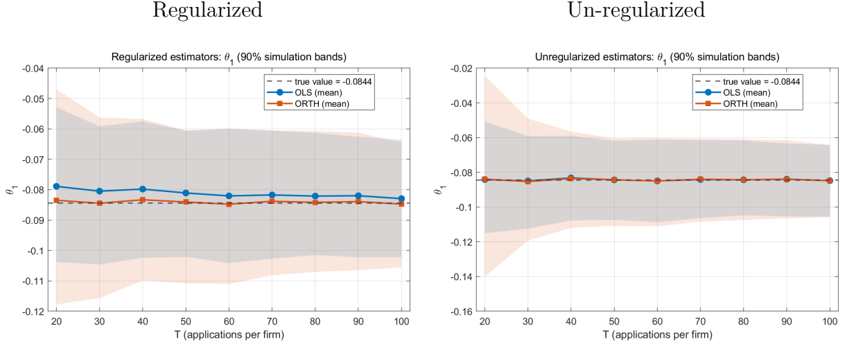
Figure 1: Monte Carlo estimates of \theta_1 as a function of T . Solid lines show the mean across simulations for OLS and ORTH; the dashed line is the true value; shaded regions are 90% simulation bands.
