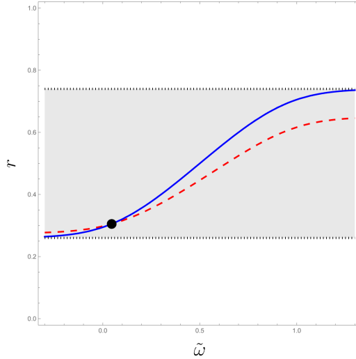
Figure 3: Solution of system (13) for \omega \sim U[0, 1] , \rho = 8 and \Delta = 0.15 : r^* \approx 0.305 , \tilde{\omega}^* \approx 0.046 . The solid blue curve is the seller's reaction, the dashed red curve is the buyer's break-even condition.
