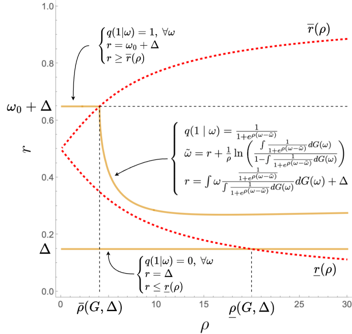
Figure 4: Equilibrium price correspondence (orange solid curve) when \omega \sim U[0, 1] and \Delta = 0.15 . Dashed red curves correspond to min and max prices compatible with interior solutions, \underline{r}(\rho) and \bar{r}(\rho) .
