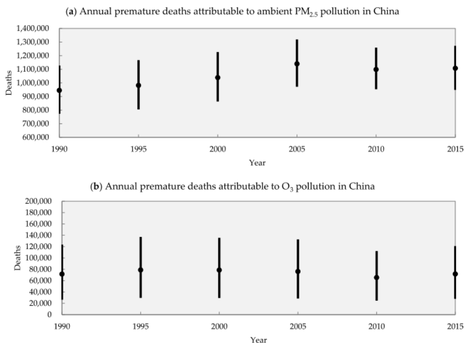
Figure 3. China's annual premature deaths attributable to PM 2.5 (a) and O 3 (b), 1990–2015. Dots show the estimated base value, bars show lower and upper bound of estimates. Based on data in the Global Burden of Disease Study 2015 [37]. Note the different scales of the vertical axes in (a) and (b).
