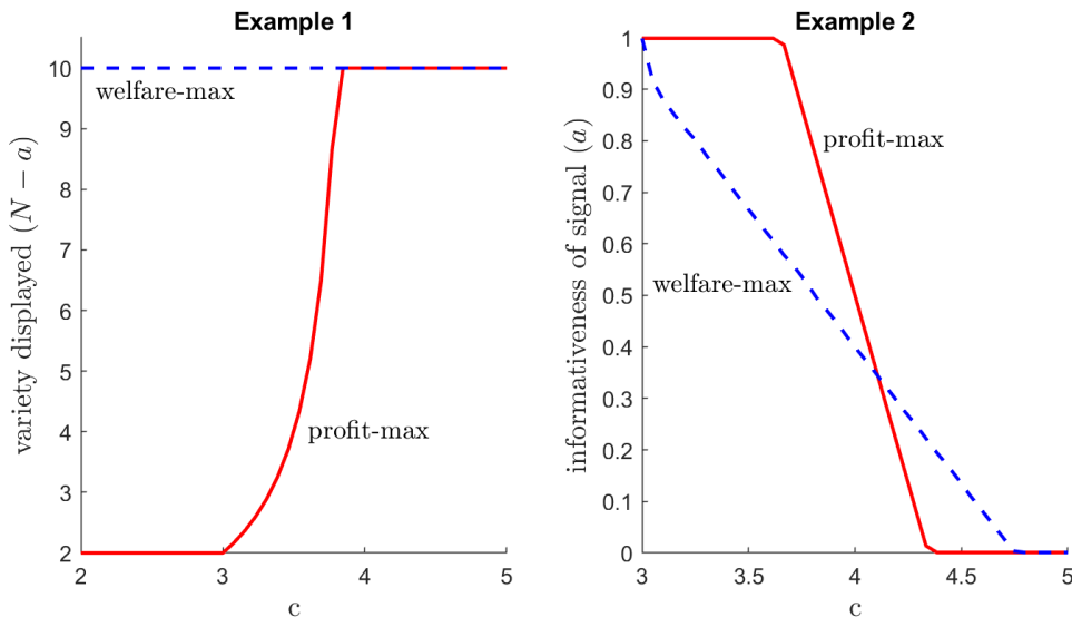
Figure 1: Governance design with exogenous proportional fee r = 0.2 : (1) Variety displayed in Example 1, and (2) Information design of Example 2. We assume V_0 = 10 , t = 2 and Q(t) is the uniform cdf with domain [0, V_0/2] .
