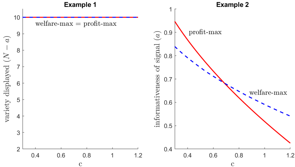
Figure 2: Governance design with endogenous proportional fees: (1) Variety displayed in Example 1, and (2) Information design of Example 2. We assume V_0 = 20 , t = 15 , and Q(t) is the uniform cdf with domain [0, V_0/2] .
