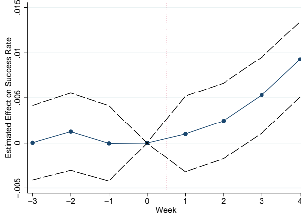
Figure 6: Week-Specific Effects
