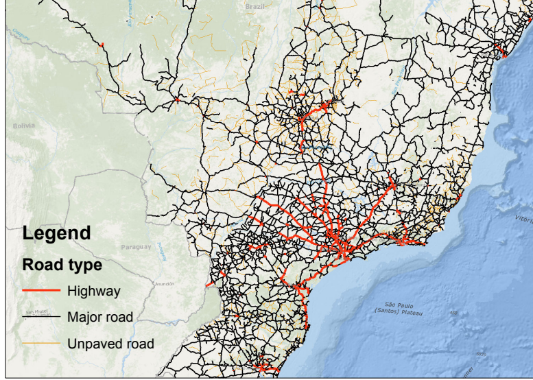
Figure 4: Road Network
