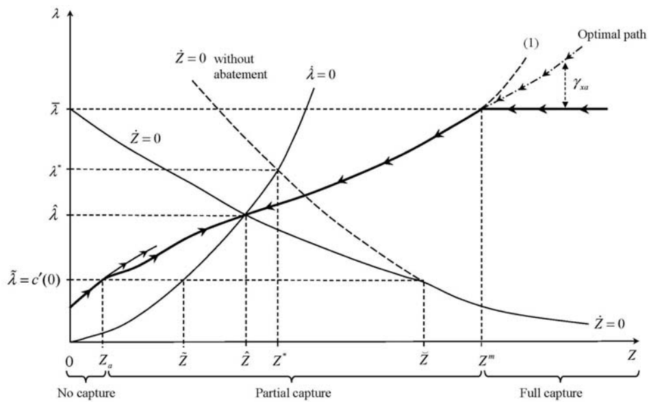
Figure 2: Phase diagram. Cheap strictly convex capture cost with c'(0) > 0 and an abundant resource.
