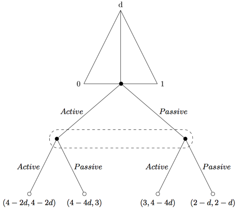
Figure 2. Extensive Form
