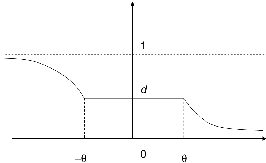
Figure 1: The function d(\cdot) .
