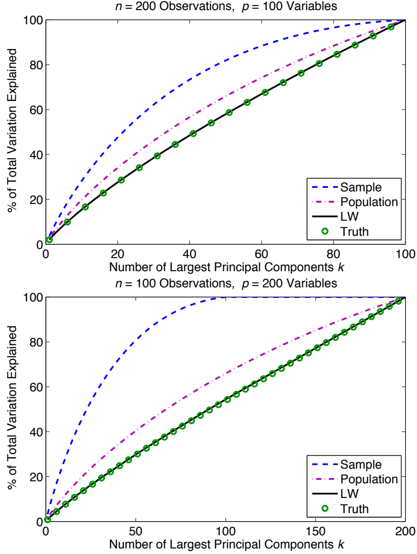
Figure 7: Comparison between different estimators of the percentage of total variation explained by the top principal components.
