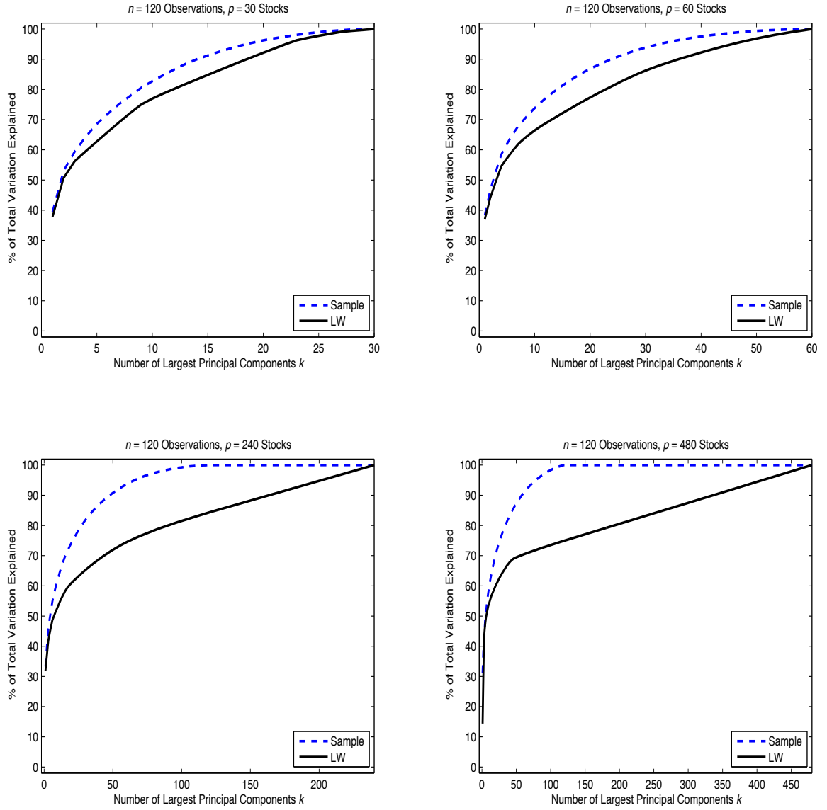
Figure 8: Percentage of total variation explained by the k largest principal components of stock returns: estimates based on the sample covariance matrix (Sample) compared to those based on nonlinear shrinkage (LW).
