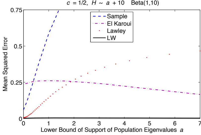
Figure 4: Effect of the condition number on the mean squared error between estimated and population eigenvalues.
