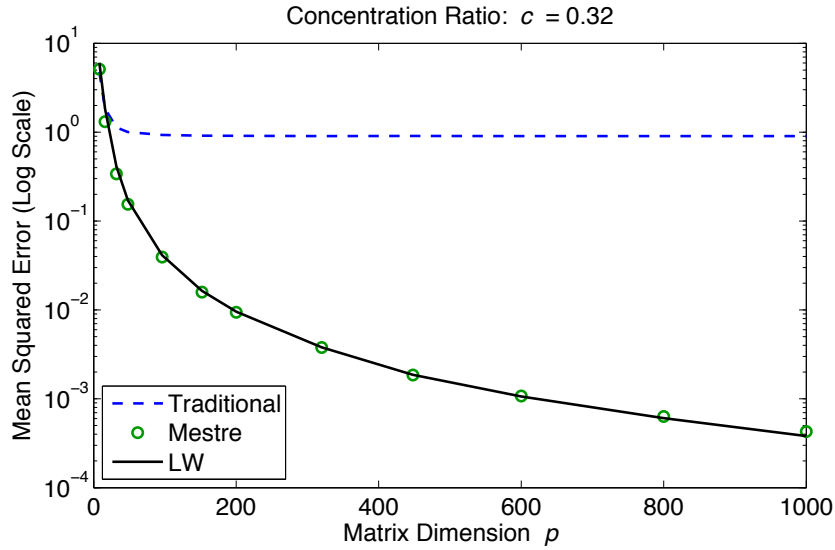
Figure 5: Convergence of estimated eigenvalues to population eigenvalues when eigenvalues are grouped into a small number of high-multiplicity clusters.
