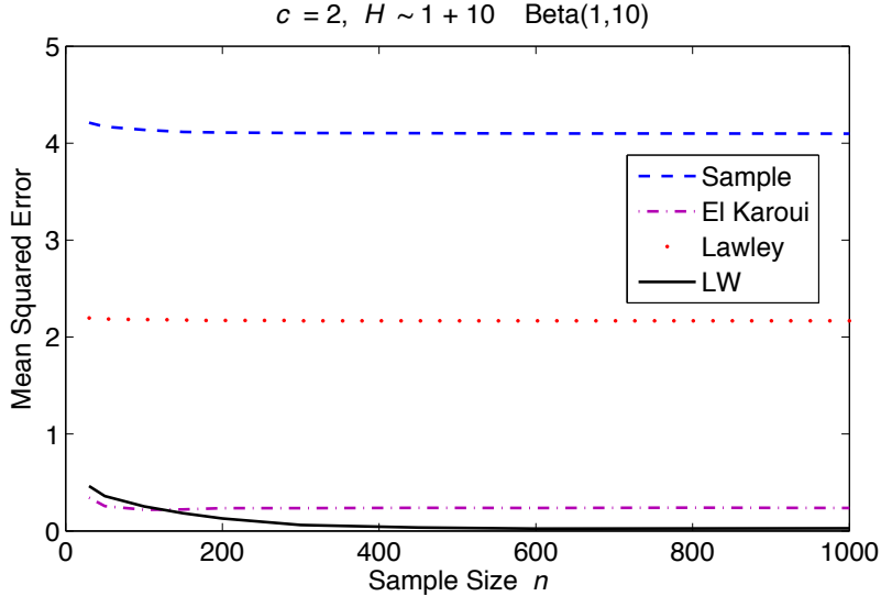
Figure 3: Convergence of estimated eigenvalues to population eigenvalues in the case where the sample covariance matrix is singular.
