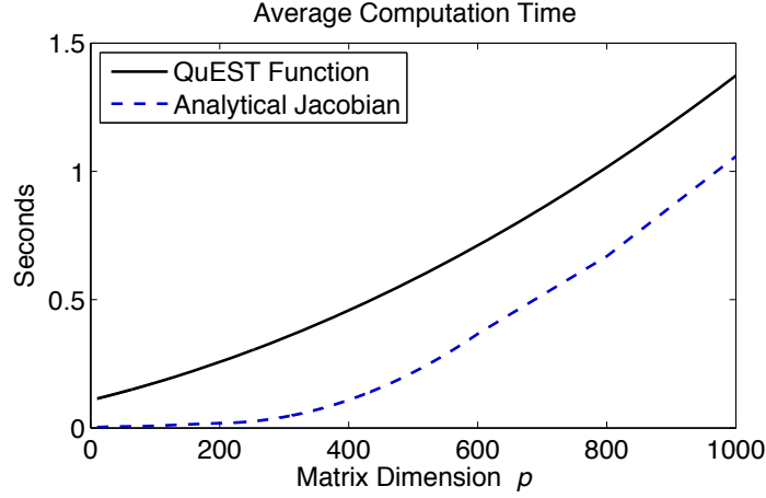
Figure 1: Average computation time for the QuEST function and its analytical Jacobian. The setup is the same as in Figure 2 below. The QuEST function and its analytical Jacobian are programmed in Matlab. The computer is a 2.4 GHz Quad-Core Intel Xeon desktop Mac.
