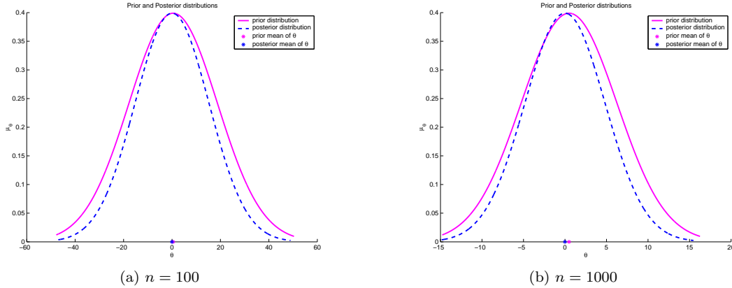
Figure 2: CASE II - prior and posterior distributions and means of \theta . The true value of \theta is 0.
