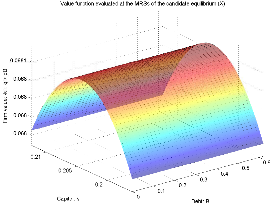
Figure 2: Value of an arbitrary firm, -k + q(k, \phi, B) + pB , as a function of k and B (for \phi = 1 ), where q(k, \phi, B) is computed using the consumers' MRSs at the equilibrium allocation. The \times in the plot represents the lower bound of the Modigliani-Miller region, i.e. B = .30615 .
