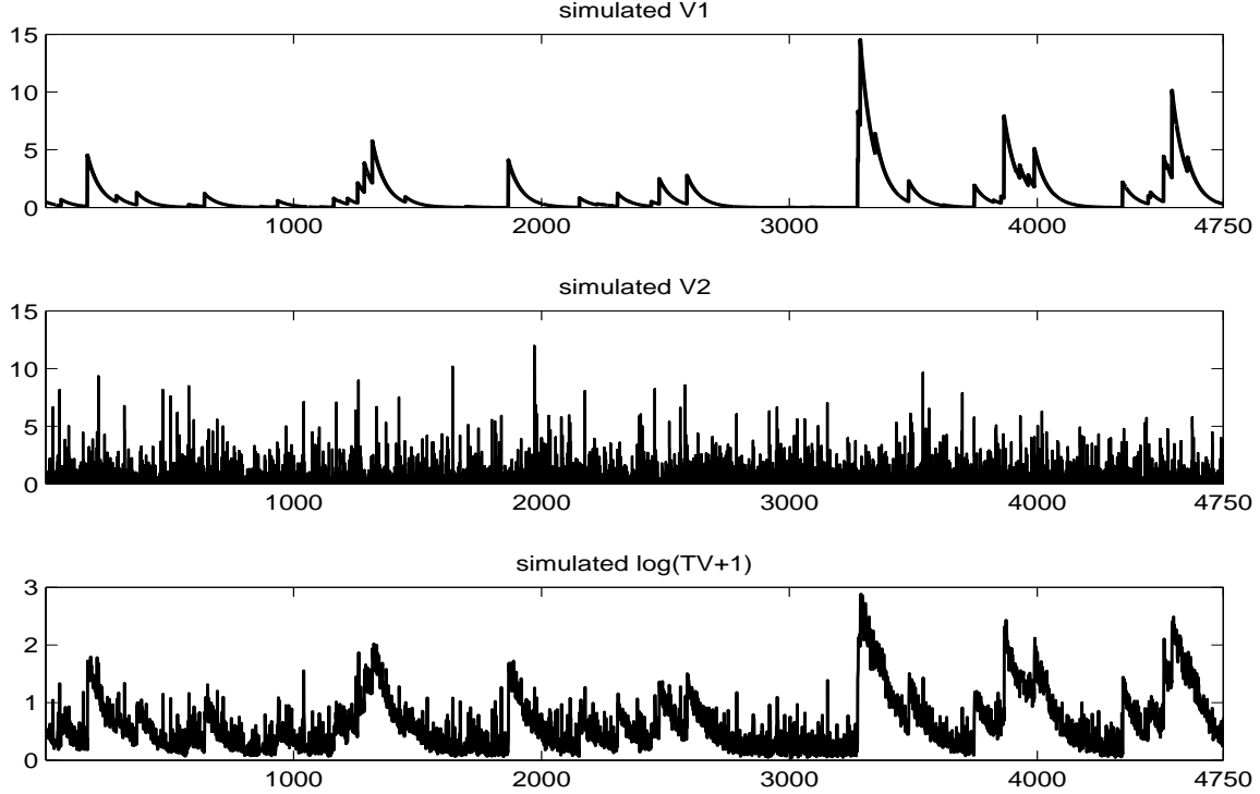
Figure 4: Simulated volatility from the estimated two-factor pure-jump model with parameter estimates reported in the last column of Table 6. The units on the horizontal axes are simulated days.
