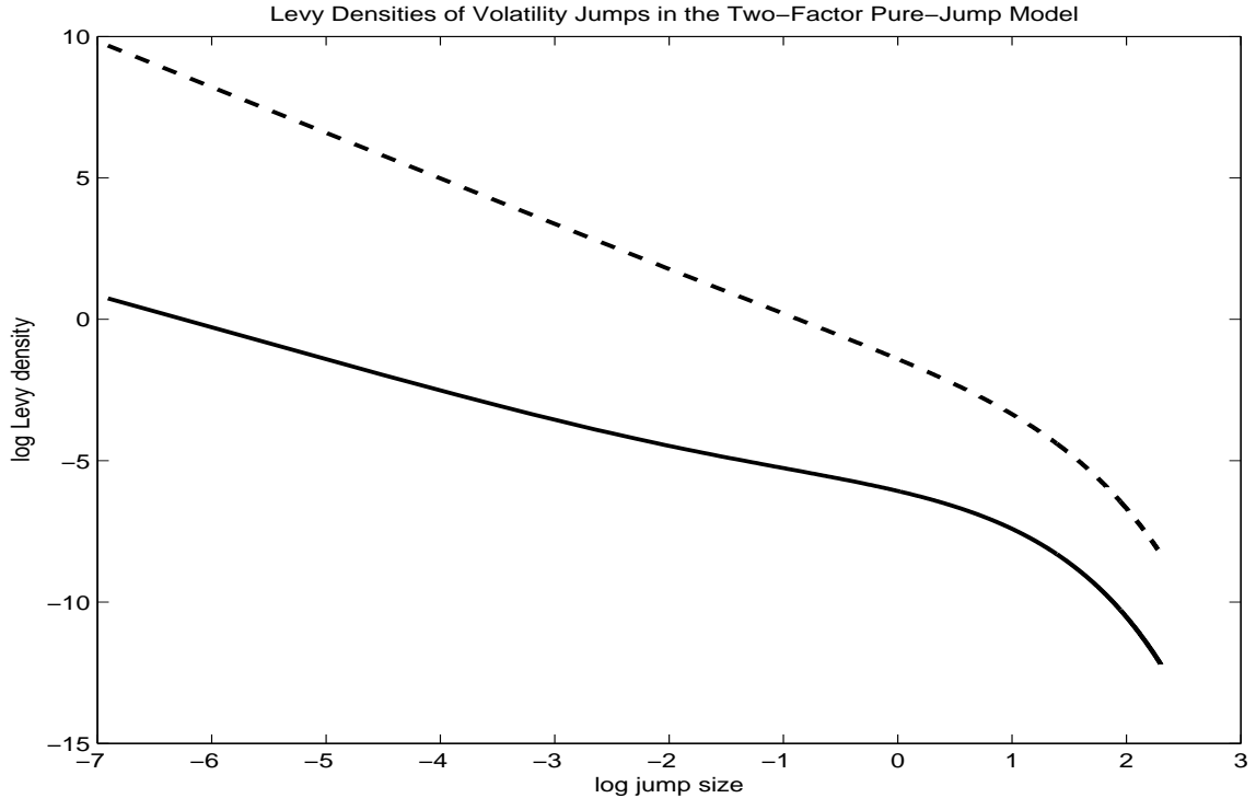
Figure 3: The Lévy densities of the volatility jumps are defined in (15) and the parameter estimates used in the calculation are reported in the last column of Table 6. Solid line corresponds to V_{1t} and dotted line to V_{2t} .
