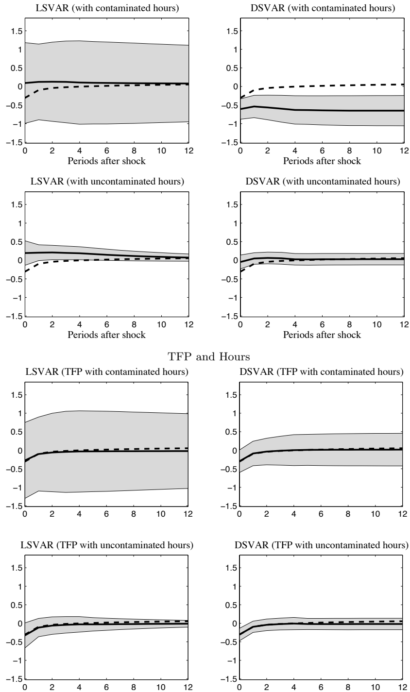
Figure 6: IRF of Hours: Labor Productivity and Hours Labor Productivity and Hours
