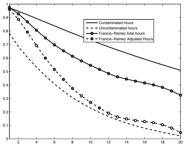
Figure 5: ACFs
