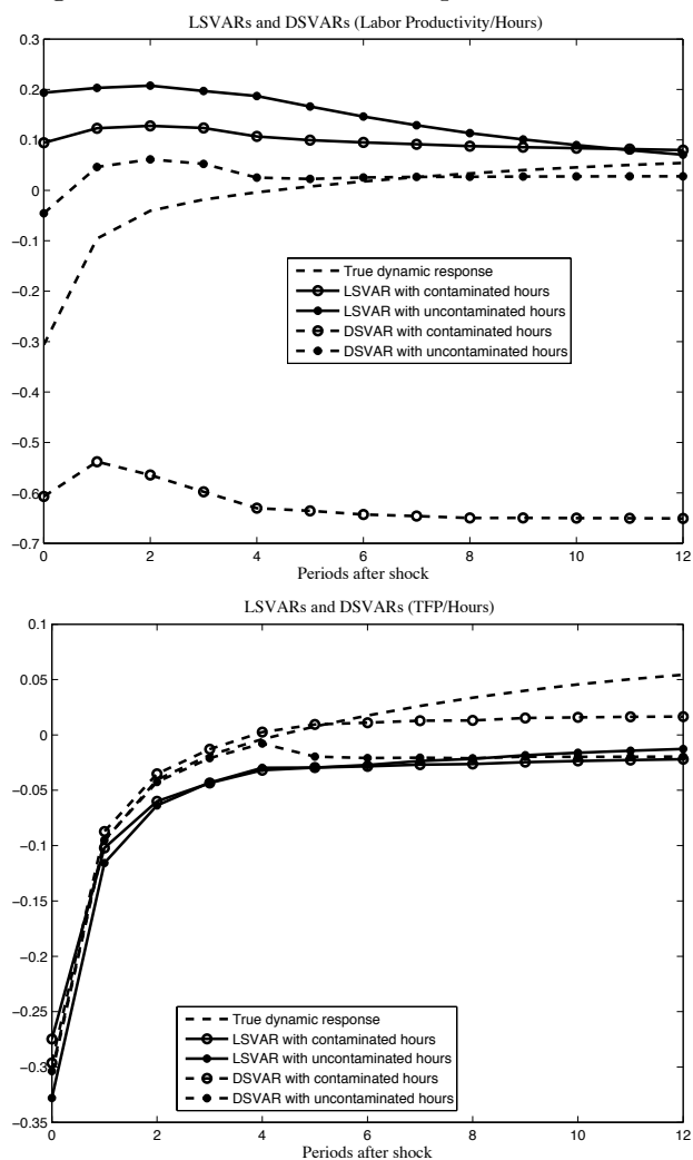
Figure 7: IRF of Hours: Comparison of SVARs
