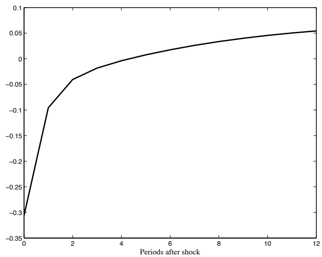
Figure 4: IRF of Hours
