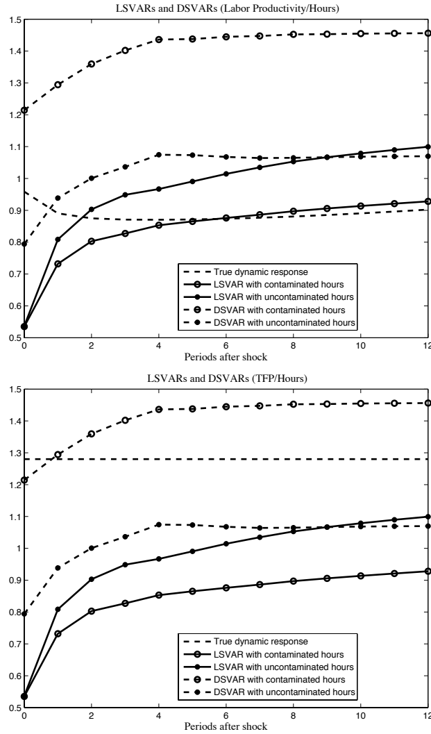
Figure 9: IRF of Productivity Measure: Comparison of SVARs
