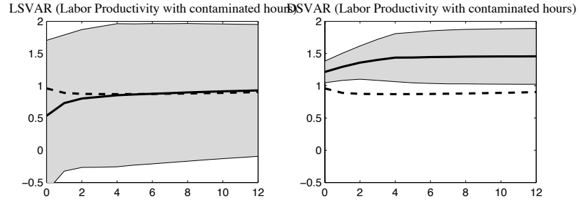
Figure 8: IRF of Productivity
