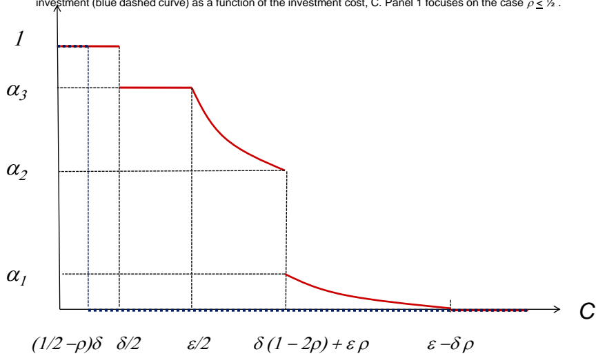
Figure 7, Panel 1: Equilibrium and utilitarian optimum when \rho \leq \frac{1}{2}
