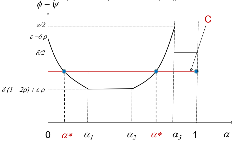
Figure 6, Panel 2. Equilibrium when \rho > \frac{1}{2} and \delta(1-2\rho) + \varepsilon\rho < \delta/2
